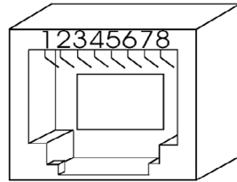
Figure 2 — RJ-45 Connector
