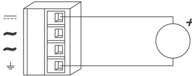
Figure 6 — DC Powered
