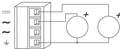
Figure 7 — Redundant DC Powered
