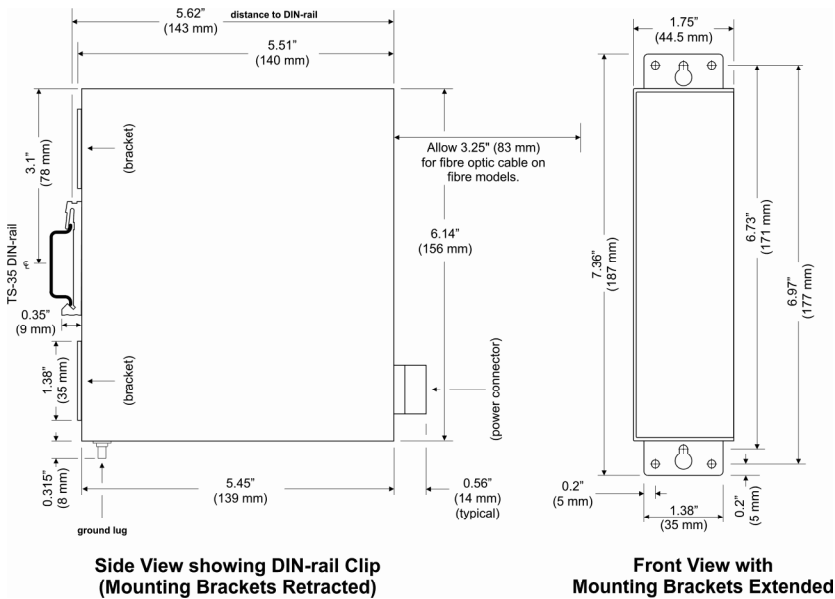
Figure 1 — EISB Dimensions
